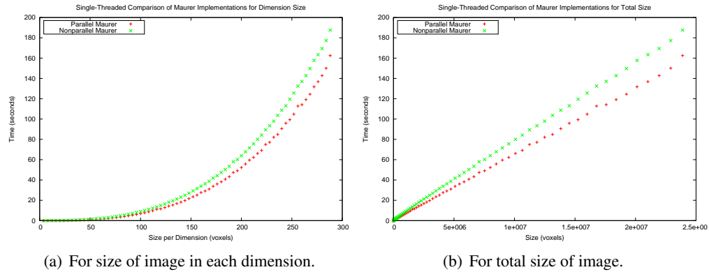
Figure 1: Comparison of run times for 3D image of our parallel Maurer implementation running with a single thread and the existing ITK Maurer implementation.
